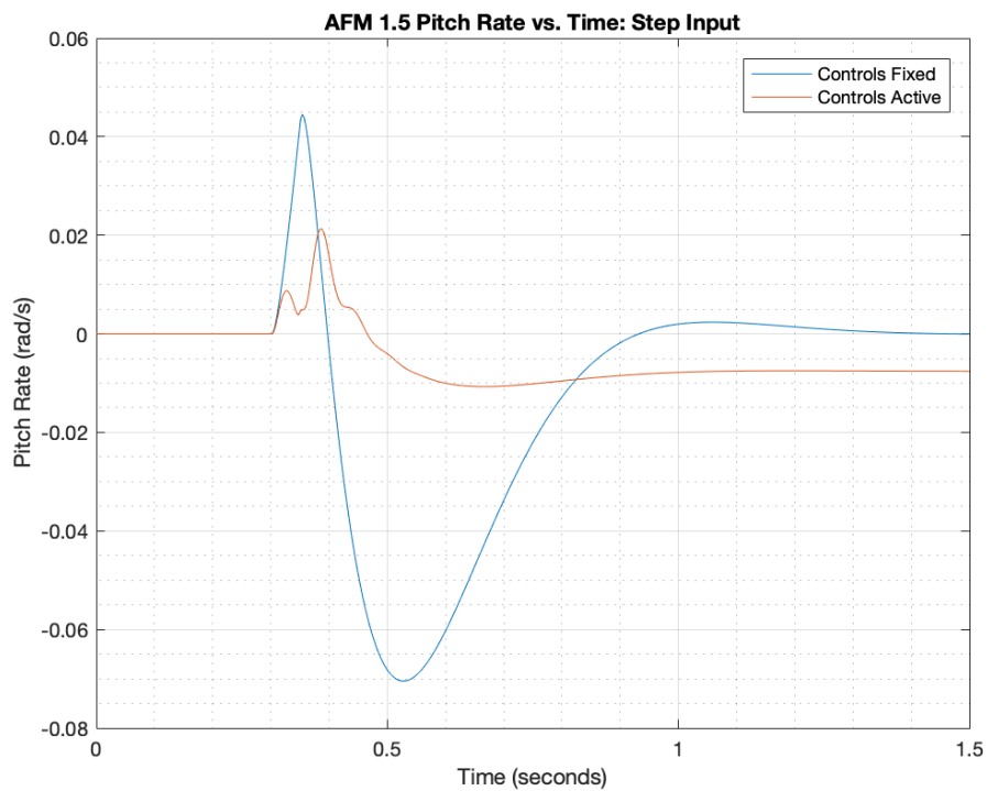
Figure 4.3 Step Gust Pitch Rate Response
