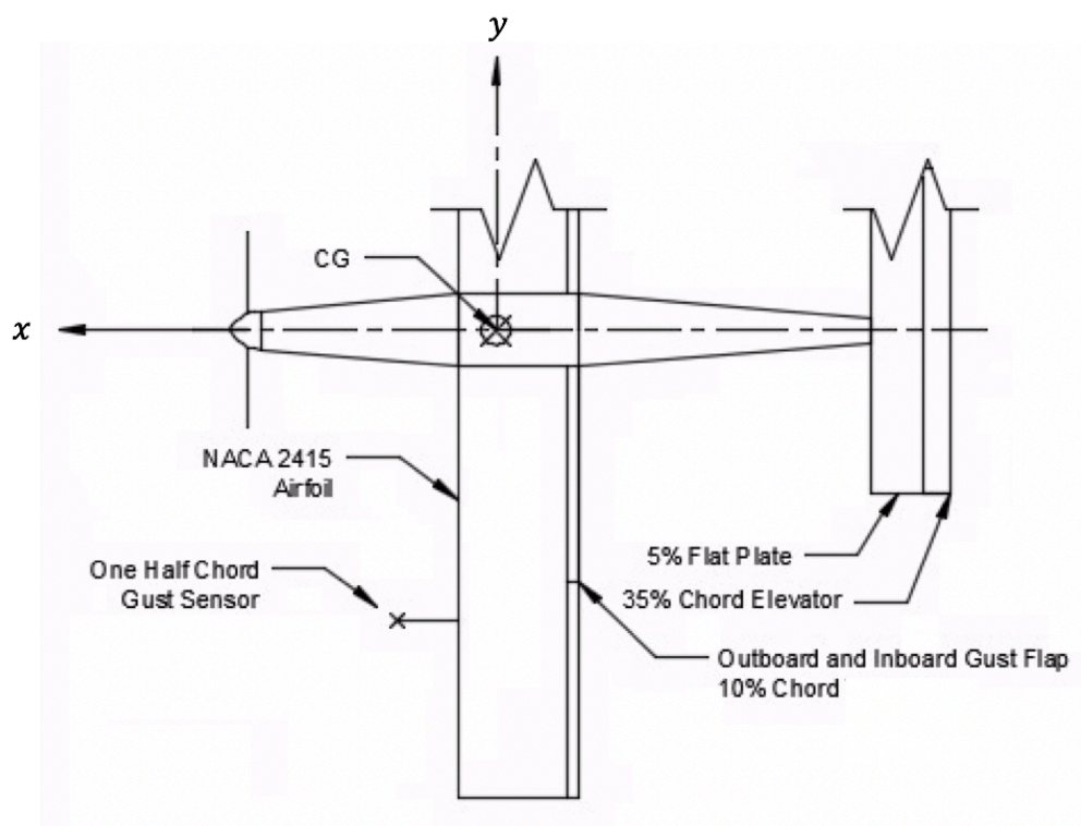
Figure 2.3 ARIS Planform
